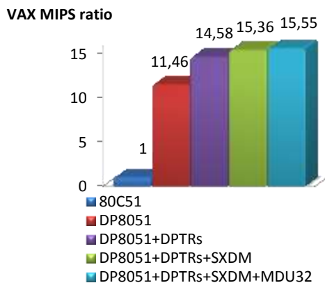
Core performance in terms of DMIPS per MHz
